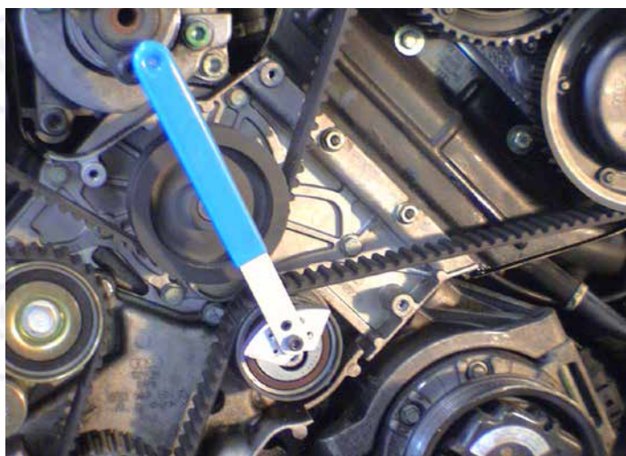
SPANNROLLENSCHLÜSSEL
